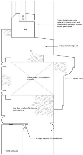
Detail at door head/fanlight
