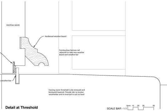
Detail at Threshold
